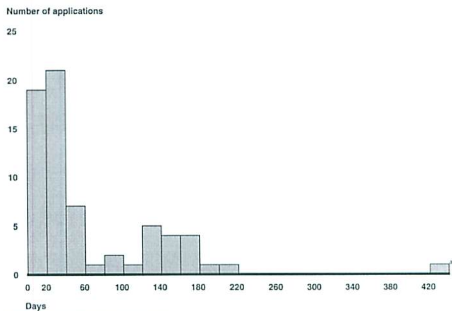
Figure 7: Distribution of Total Days from Transmission by Post to Response from State
